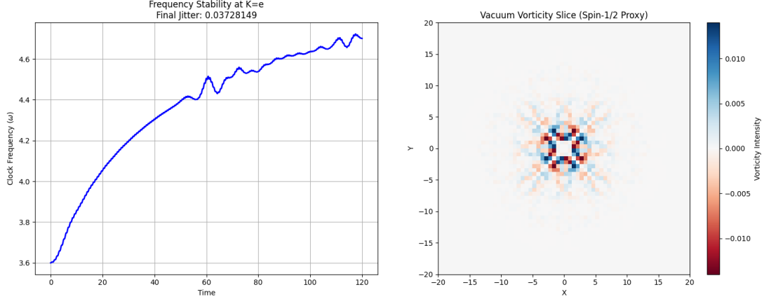
Figure 2: 3D Verification of Stability and Spin. Left: The temporal evolution of the internal clock frequency shows clear convergence, validating the Euler coupling hypothesis. Right: A 2D cross-section of the vacuum vorticity field ( \nabla \times \mathbf{J} ) surrounding the core. The emergence of this structured circulation pattern provides direct numerical evidence for the hydrodynamic origin of spin discussed in Section 10.
